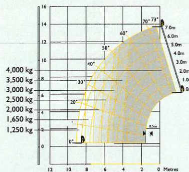
540-140 Stabilisers extended
