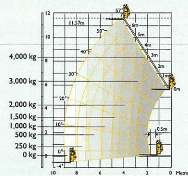
540-170 Stabilisers retracted
