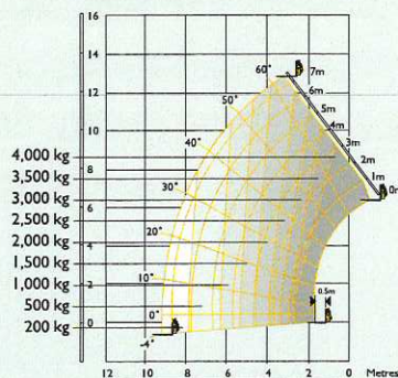
540-140 Stabilisers retracted
